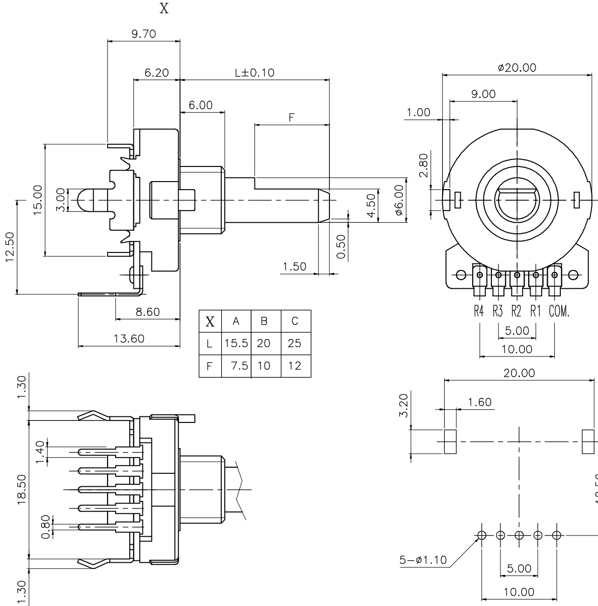
Mounting hole detail
